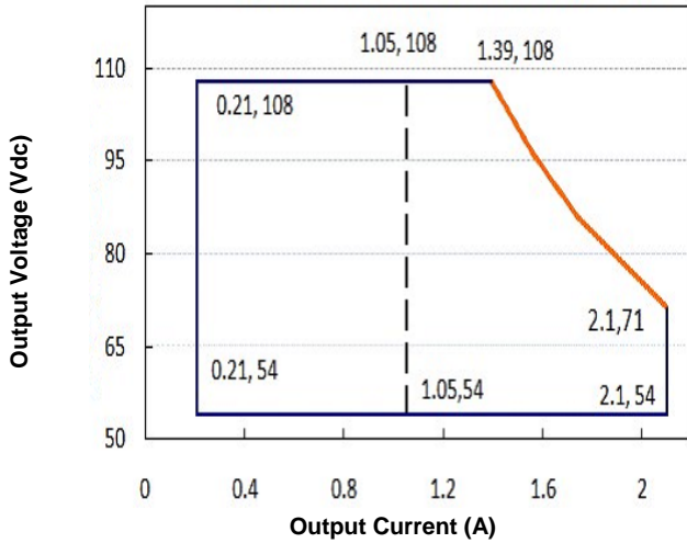
Figure 3: Typical V-I Characteristic Curve (LUB150X-108CP)
