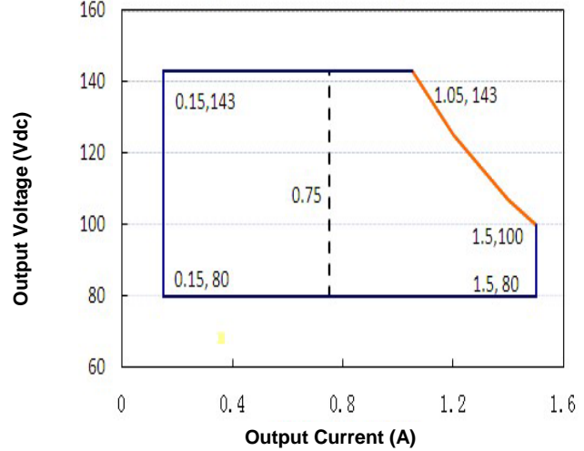
Figure 4: Typical V-I Characteristic Curve (LUB150X-143CP)
