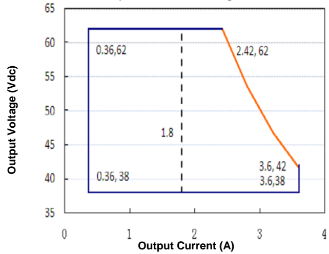
Figure 2: Typical V-I Characteristic Curve (LUB150X-062CP)
