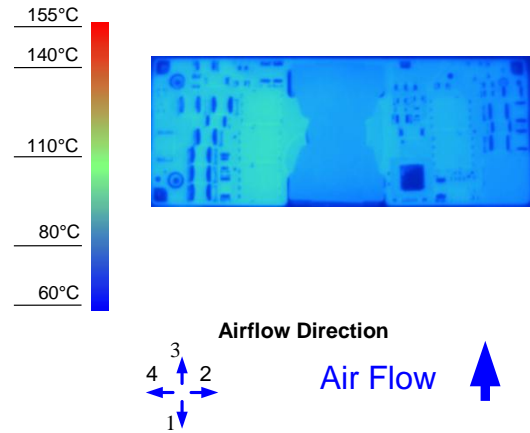
Figure 8. Thermal Image for Airflow Direction 3 (15A output, 55°C ambient, 200 LFM, typical V_{in} , open frame, socket interface)
