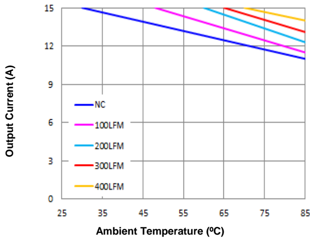
Figure 7. Current Derating Curve for Airflow Direction 3 (Ref. Fig. 8 for Airflow Direction; V_{in} = 48V , open frame)
