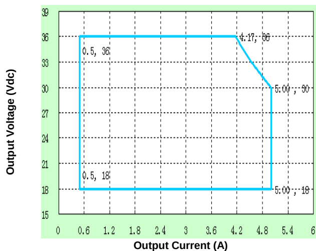
Figure 1: Typical V-I Characteristic Curve (LHA150X-036C)
