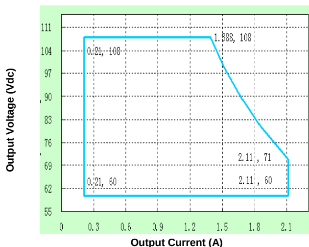
Figure 3: Typical V-I Characteristic Curve (LHA150X-108C)
