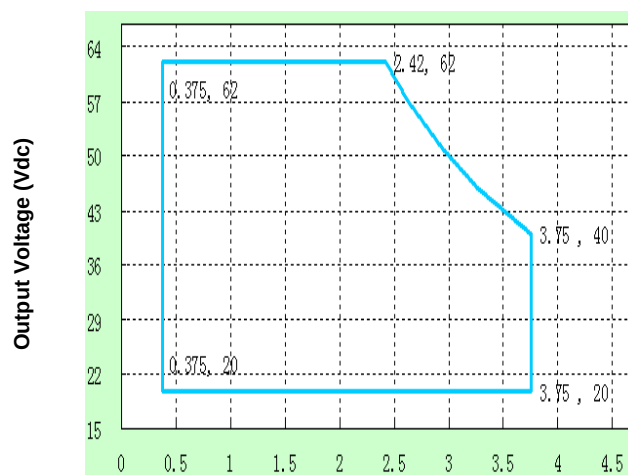
Figure 2: Typical V-I Characteristic Curve (LHA150X-062C)
