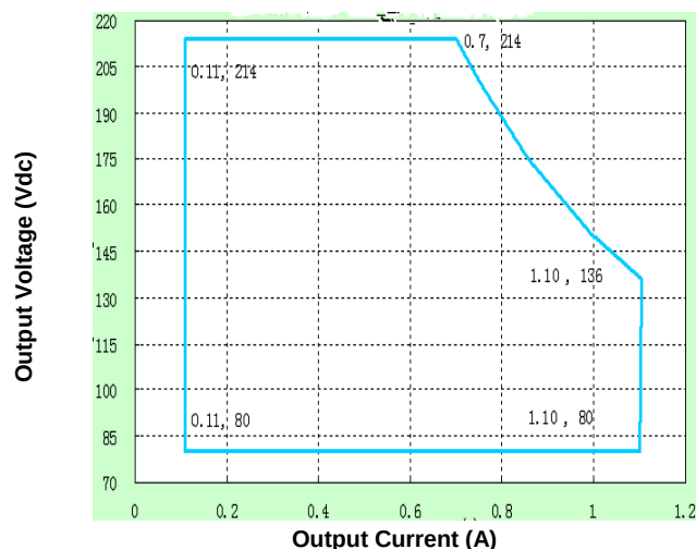
Figure 4: Typical V-I Characteristic Curve (LHA150X-214C)
