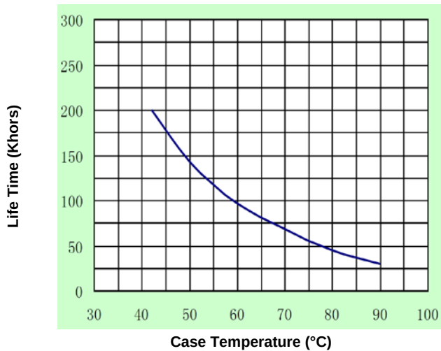
Figure 11: Life Time vs. Case Temperature
