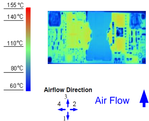
Figure 12. Thermal Image for Airflow Direction 3 (10A output, 55°C ambient, 200 LFM, typical V_{in} open frame unit)
