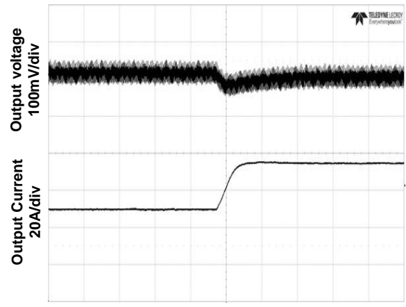
Time - t (500μs/div) Figure 6. Transient Load Response Top: Output voltage deviation Bottom: Load current step (+25% full load) Test Cond.: Output current at 50% full load, typical Vin, slew rate 0.1A/μs
