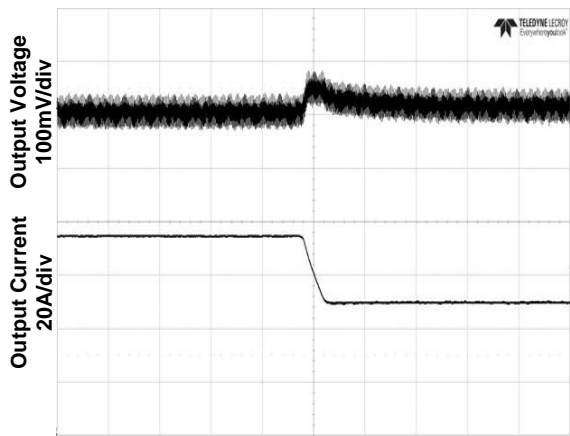
Time - t (500μs/div) Figure 5. Transient Load Response Top: Output voltage deviation Bottom: Load current step (-25% full load) Test Cond.: Output current at 50% full load, typical Vin, slew rate 0.1A/μs
