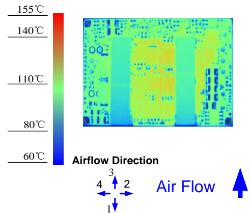
Figure 8. Thermal Image for Airflow Direction 3 (93A output, 55°C ambient, 200 LFM, typical Vin, open frame unit using soldering interface)
