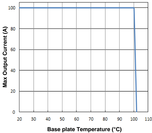
Figure 9. Current Derating Curve for Base plate (typical vin with Base plate; solder interface)
