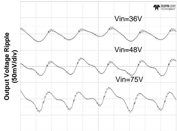
Time - t (2μs/div) Figure 4. Output Ripple Voltage at Full Load
