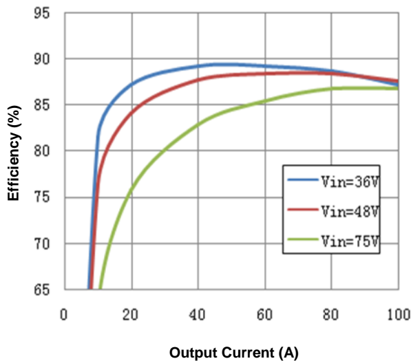
Figure 1. Efficiency vs. Load Current ( 25^\circ\text{C} )
