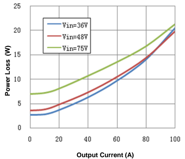
Figure 2. Power Loss vs. Load Current
