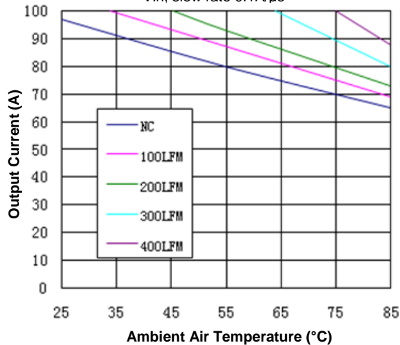
Figure 7. Current Derating Curve for Airflow Direction 3 (Ref. Figure 8 for Airflow Direction; typical Vin, open frame unit using soldering interface)
